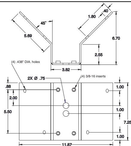
ACA2 Dimensions
