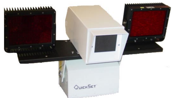
A QuickSet QPT-90 Pan Tilt Motor is integrated with two Extreme SuperLED Infrared Illuminators using the EXMB.055 Bracket.
